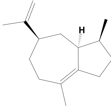
\alpha - bulnesene
