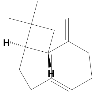
\beta - caryophyllene
