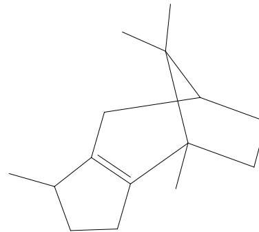
\beta - patchoulene
